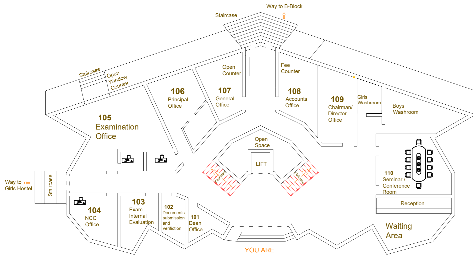
Ground Floor
